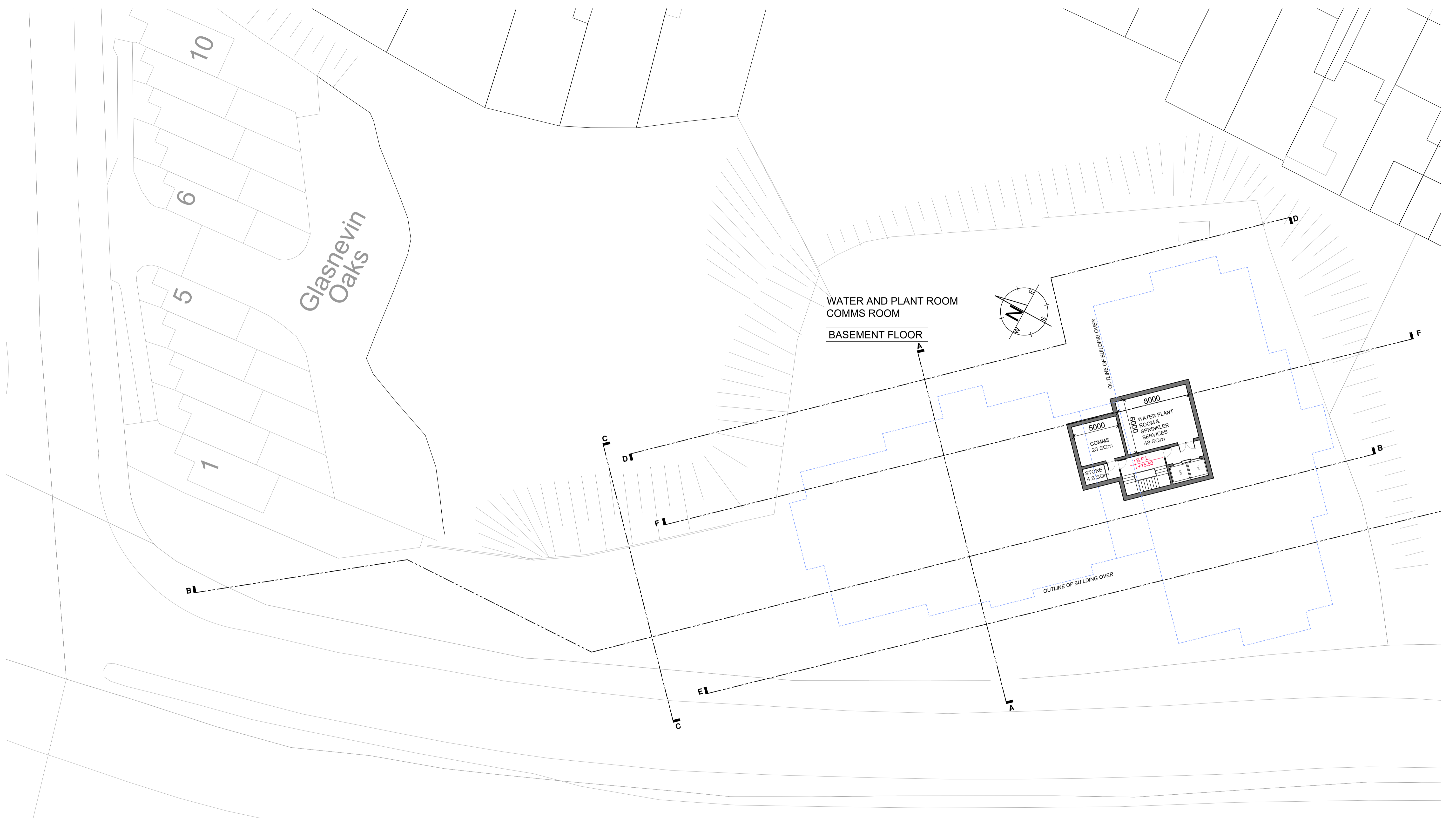
BASEMENT PLAN WITH SITE . . . . Scale 1:200
